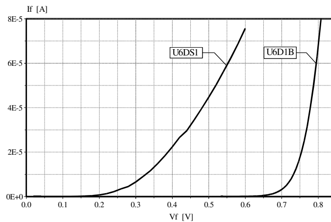
Forward characteristic
