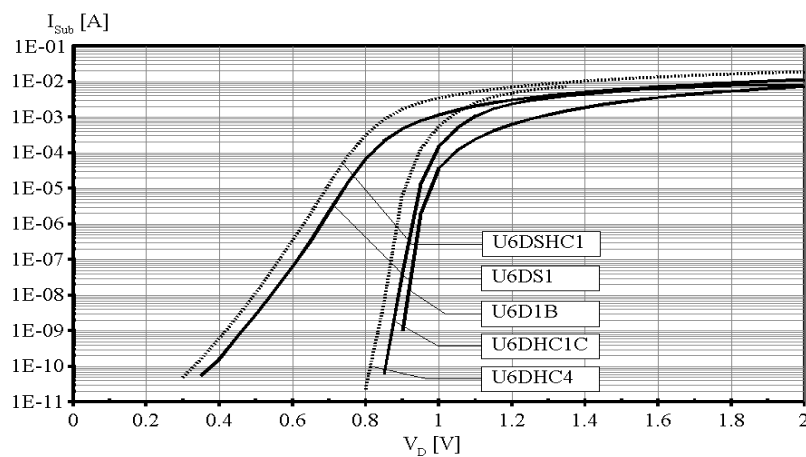
Substrate currents for PN and Schottky diodes
